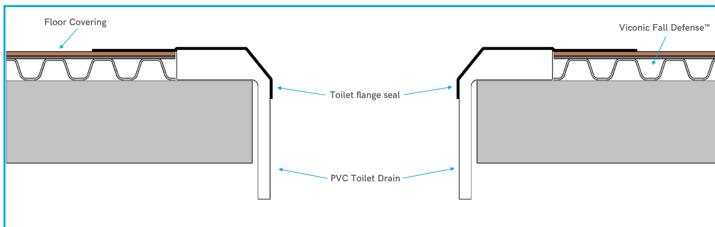
Viconic toilet drain assembly cross section. Toilet flange seal should be installed above the floor covering
