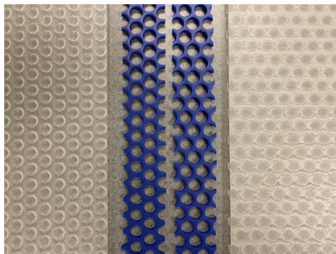
Step 2: Cut strips of subsurface support for each panel, ensuring the orientation of the subsurface support matches the orientation of the Viconic cone layer
